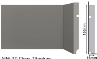
496 RP Cinza Titanium Titanium Gray Skirting Board Zócalo Gris Titano
