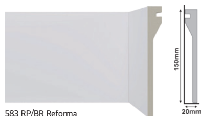
582 RP/BR Reforma White Overlapping Skirting Board Zócalo Blanco Reforma
